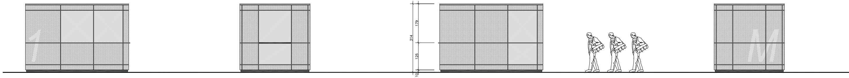
"LA MACHINE" / PAVILLON GLACIER / FERME ELEVATION 1
